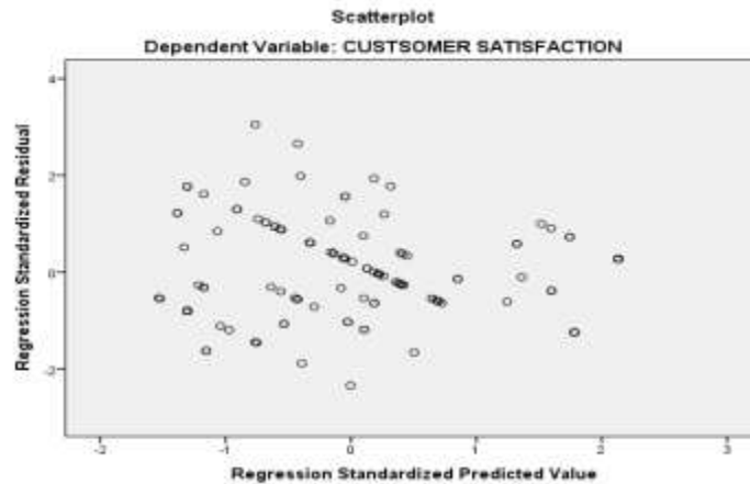
Figure 2. Normality Test
