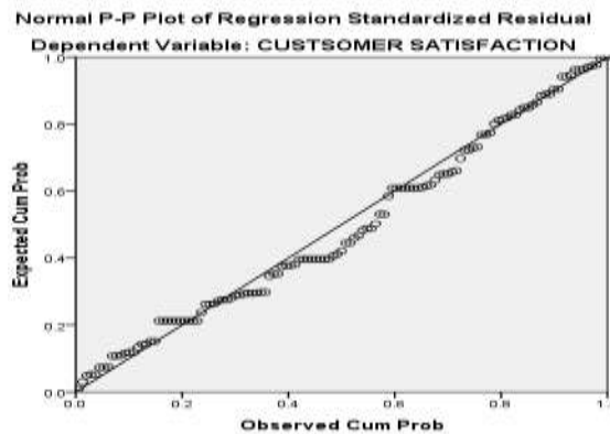
Figure 1. Normality Test
